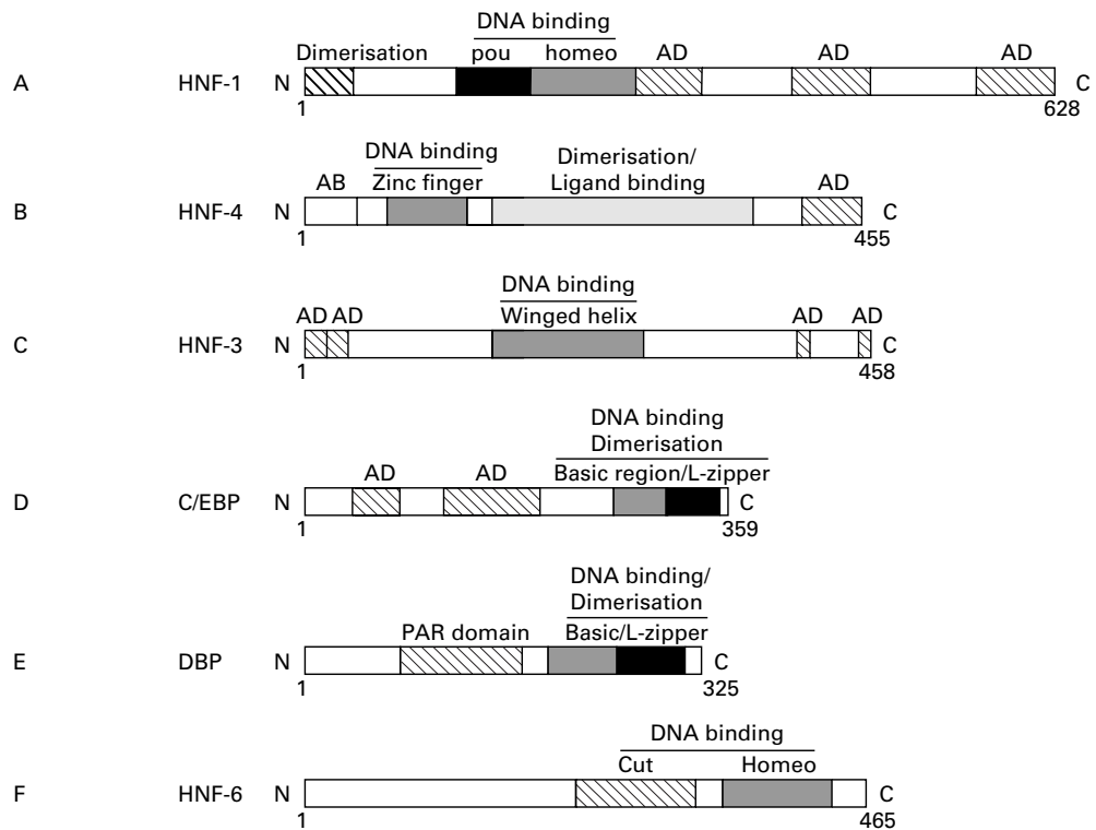
Figure 1 Schematic representation of liver enriched transcription factor proteins. (A) HNF-1 contains highly conserved dimerisation, POU (sequence specific recognition), and homeo domains and non-conserved transcriptional activation domains (AD). (B) HNF4 contains highly conserved DNA binding (zinc finger motif) and dimerisation/ligand binding domains, and non-conserved variant A/B as well as transcriptional activation domains (AD). (C) The HNF-3 family contains a highly conserved DNA binding domain (winged helix motif) and two transcriptional activation domains in the C-terminal and N-terminal regions, respectively. (D) The C/EBP family contains a highly conserved basic region, leucine zipper motif, and two transcriptional activation domains (AD). (E) DBP has a similar structure to C/EBP but it also has a PAR domain. (F) HNF-6 contains two different DNA binding domains: cut and homeo domains.
